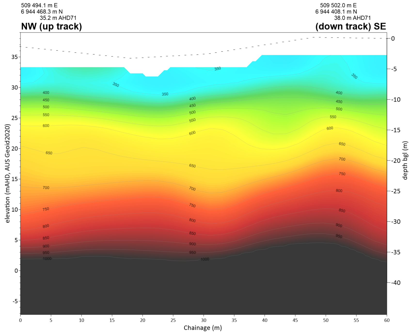
Seismic Line MASW AU-GP 116
